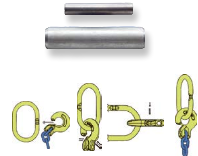
Assembly: C-coupling - C-grab/C-lok with MF
