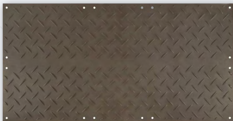
TUFFTRAK ALTURNAMAT HIGH LOAD 120 ton, 4 ft x 8 ft HSI # 1013-17892
